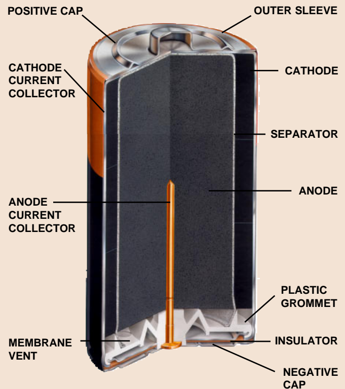
DURACELL® cylindrical alkaline cell.
